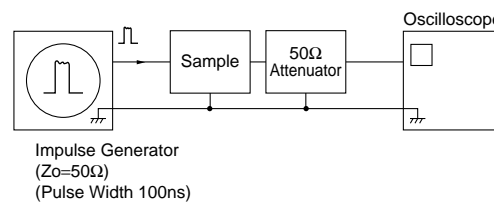
[TESTING CIRCUIT]
