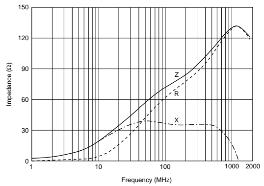
BLM03AG700SN1
